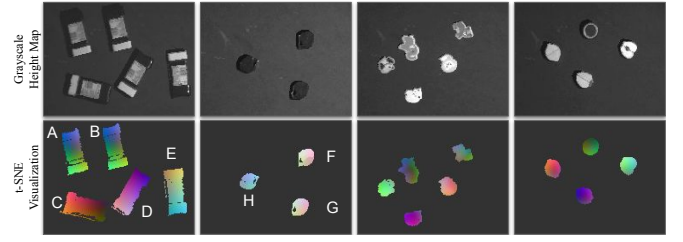
Fig. 7. The t-SNE embedding visualizations of object descriptors for different kits show that the descriptors have learned to encode rotation (A, B, C), spatial correspondences (identical points on A and B share similar descriptors) and object identity (all zoo animals have unique descriptors).
